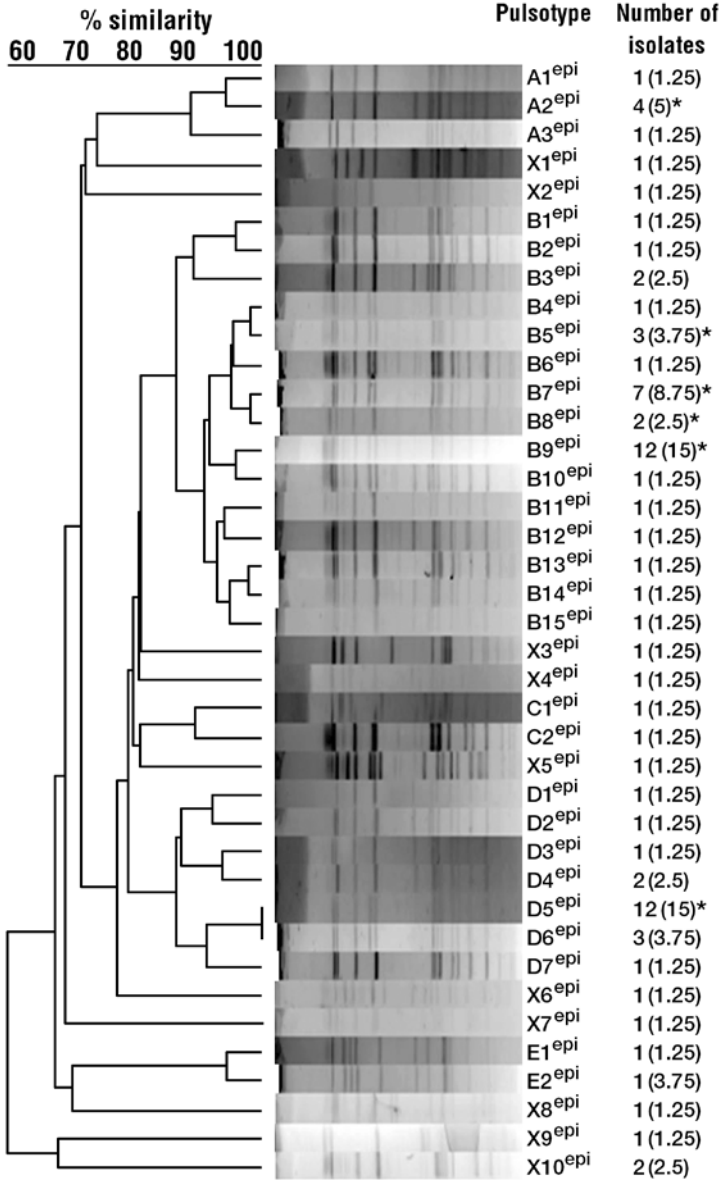
Fig. 1. Pulse field gel electrophoresis analysis of S. epidermidis A1 epi , A2 epi etc. indicate – A1 sub-pulsotype of S. epidermidis ; * occurrence of sub-pulsotype in two or more provinces; figures in the parenthesis indicate occurrence of the given sub-pulsotype in per cent.
